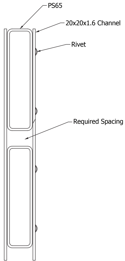
SECTION F-F SCALE 1 : 1
